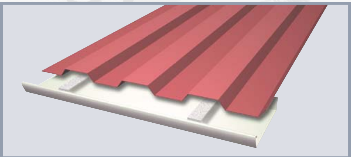
If practical, internal gutter brackets should be positioned under the crests of the profile.
